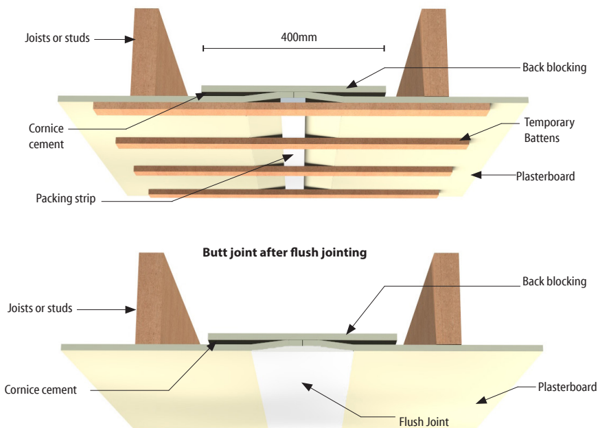
Back blocking using temporary battens and packer to create a tapered edge
