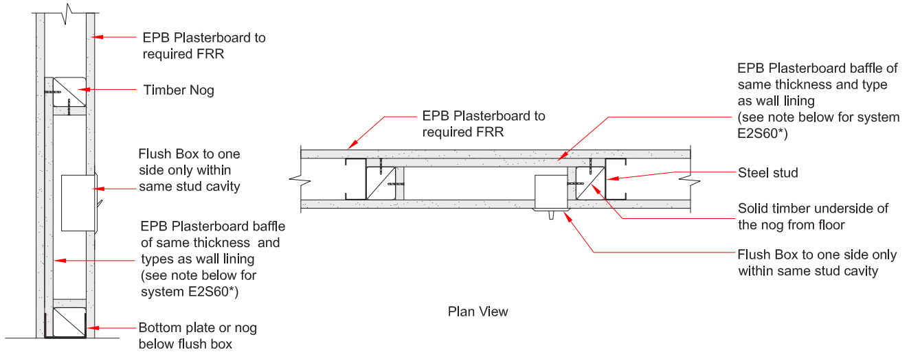
Side Elevation
