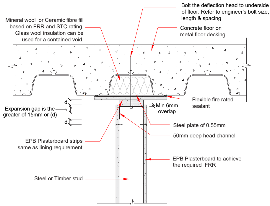
ComFlor® Detail for Wall to Profile Junction
