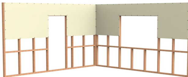
Horizontal Fixing
