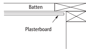
TIMBER BATTEN DETAIL (PARALLEL TO BATTEN)
