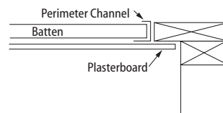
STEEL BATTEN DETAIL (PARALLEL TO BATTEN)
