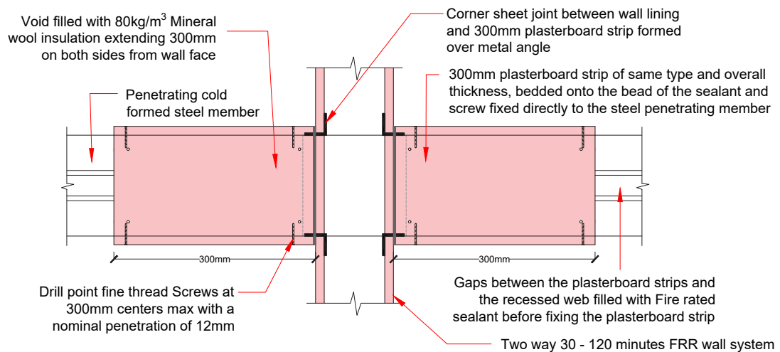
Section AA-Two way FRR wall
