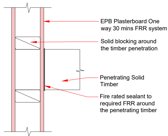
Section AA-One way FRR
